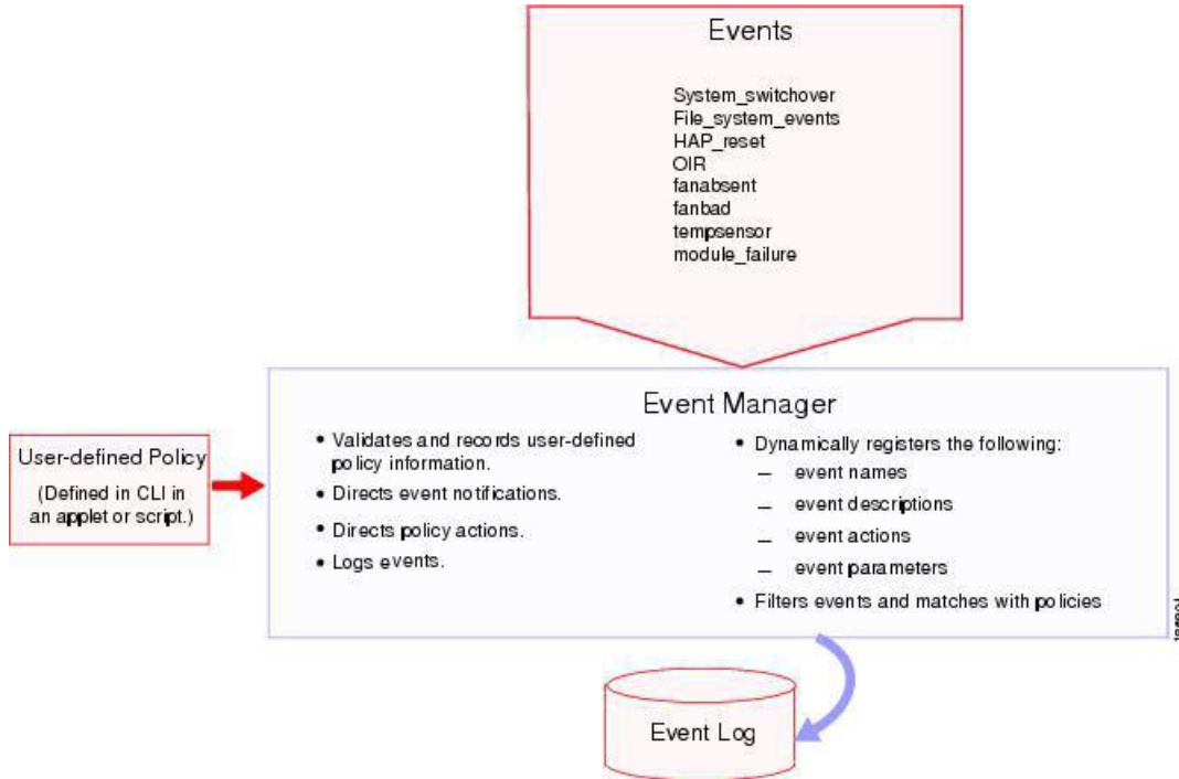
Figure 3 EEM Overview
