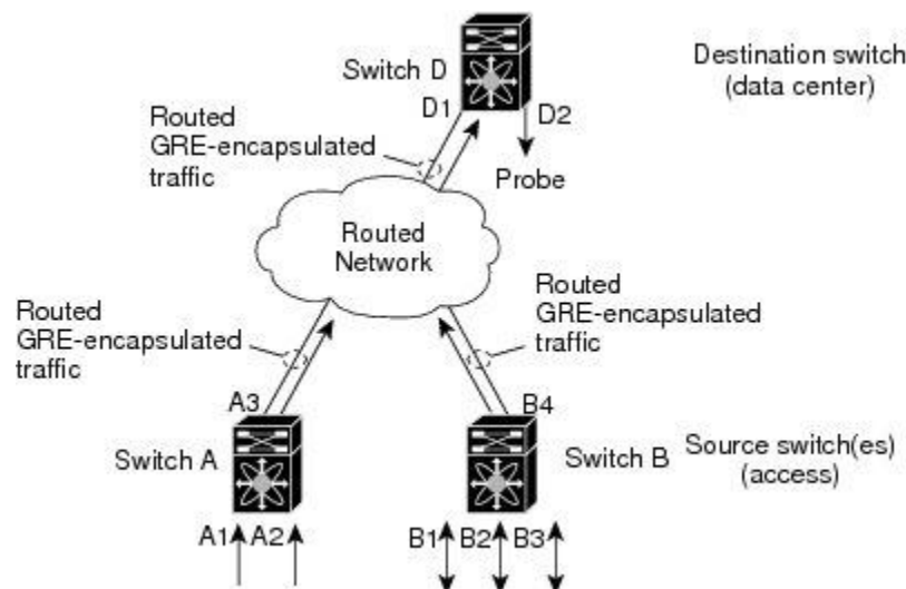
Figure 6 ERSPAN Configuration
